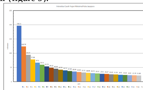
Figure 9. Mononobe method rainfall intensity
